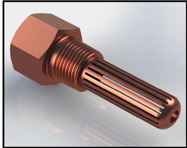
FF™ Adaptor to be used where debris is excessive
